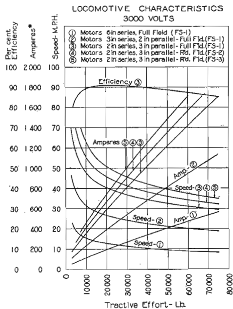
FIG. 3—LOCOMOTIVE CHARACTERISTIC CURVES
