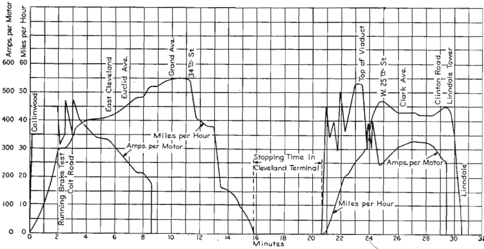
FIG. 4—SPEED-CURRENT-TIME CURVES FOR "THE 20TH CENTURY LIMITED" FROM COLLINWOOD TO LINNDALE, DEC. 2, 1931. TRAILING TONS, 1,100. CLEVELAND UNION TERMINALS ELECTRIFICATION
