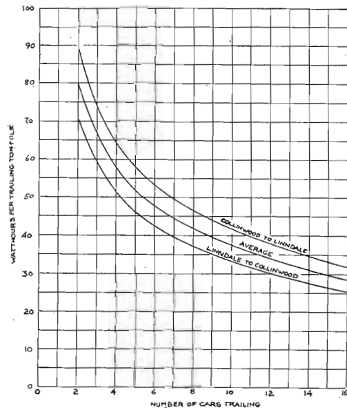
FIG. 5—ENERGY CONSUMPTION CURVES
