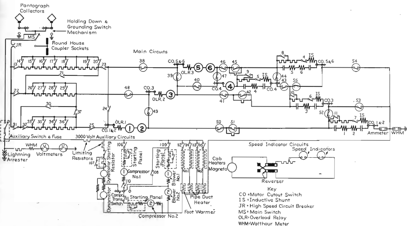
FIG. 2—MAIN AND AUXILIARY CIRCUITS FOR CLASS 2 - C + C - 2 - 300/408 - 6GE278C, 3,000-VOLT PASSENGER LOCOMOTIVE, SCHEMATIC CONNECTION DIAGRAM, FOR CLEVELAND UNION TERMINALS CO., CLEVELAND, OHIO
