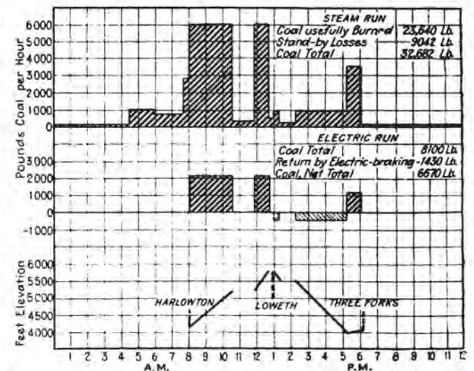
COAL CONSUMPTION COMPARISON ON IDENTICAL RUNS
